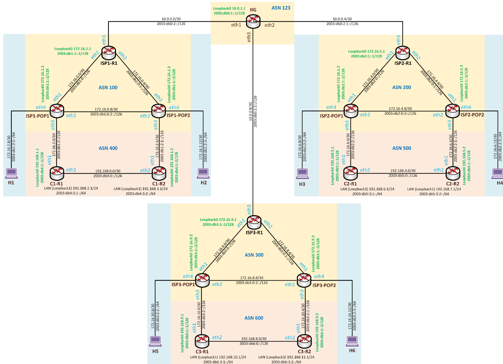
bdNOG11 IPv6 Routing Workshop on MikroTik RouterOS – LAB Topology
